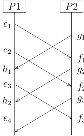
Fig. 3. A prefix of an infinite communication scenario that cannot be decomposed into finite MSCs.
