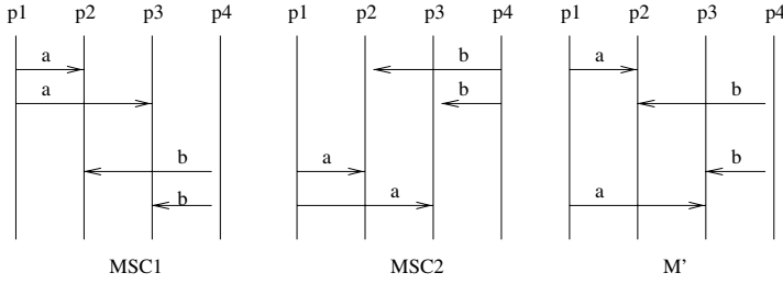
Fig. 1. Weak Inference
