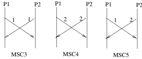
Fig. 3. Safe realizability
