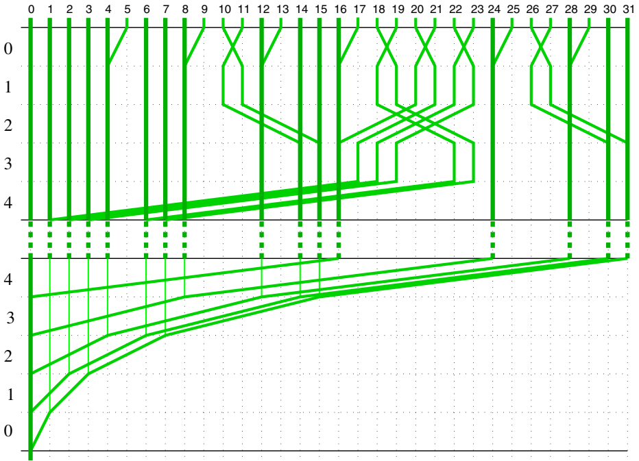
Fig. 3. Coherent row-broadcasting on RBF_5' in 13 rounds. Indicated are the used connections. The thickest lines give the packets that are not delayed. The intermediate lines, give packets that are delayed once. The thinnest lines, only occurring in the lower half, indicate packets that are delayed twice. Thus, the lower half takes 7 and the upper half 6 rounds.
