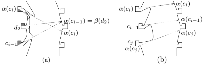
Fig. 7. Proof of Lemma 9. (a) Case 1. (b) Case 2.
