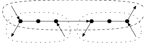
Fig. 6. The gadget ensuring consistency for a variable. If there are two positive occurrences of the variable, the ticked edges corresponding to those occurrences are represented by the parts enclosed in the dotted curves and the ticked edge corresponding to the negative occurrence is represented by the part enclosed in the dashed curve. If there are two negative occurrences, the rôles are reversed.
