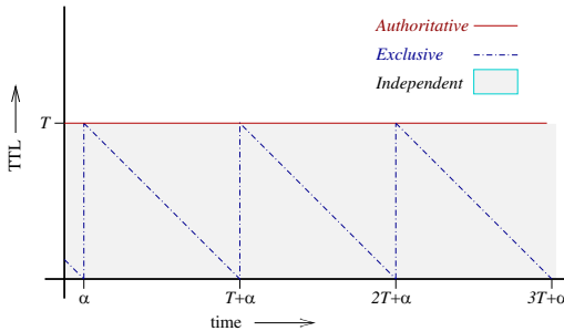
Fig. 2. TTL obtained through different types of sources. AUTH source always provides zero age and TTL of T . EXC source (shown with displacement \alpha ) provides age that cycles from 0 to T and thus TTL which cycles from T to 0. IND source provides at each point in time age drawn independently from U[0, T] and thus TTL drawn from U[0, T] .
