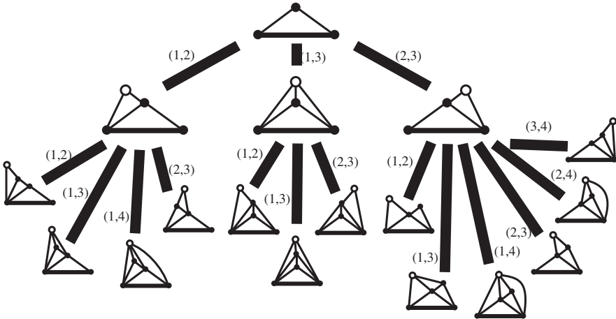
Fig. 2. Genealogical tree T_5 .
