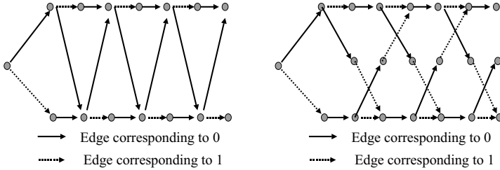
Fig. 2. Rounding graphs for \mathcal{I}_2 (left drawing) and \mathcal{I}_3 (right drawing).
