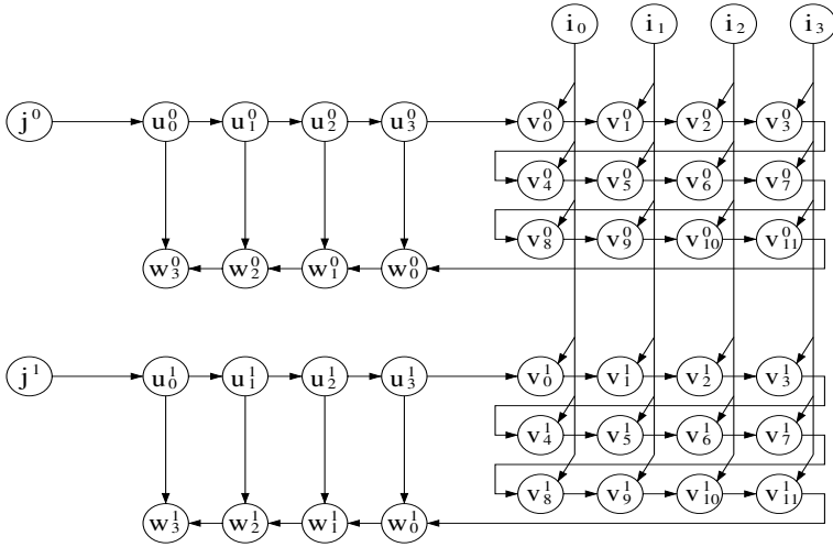
Fig. 2. The CDAG G_{3,4}^2
